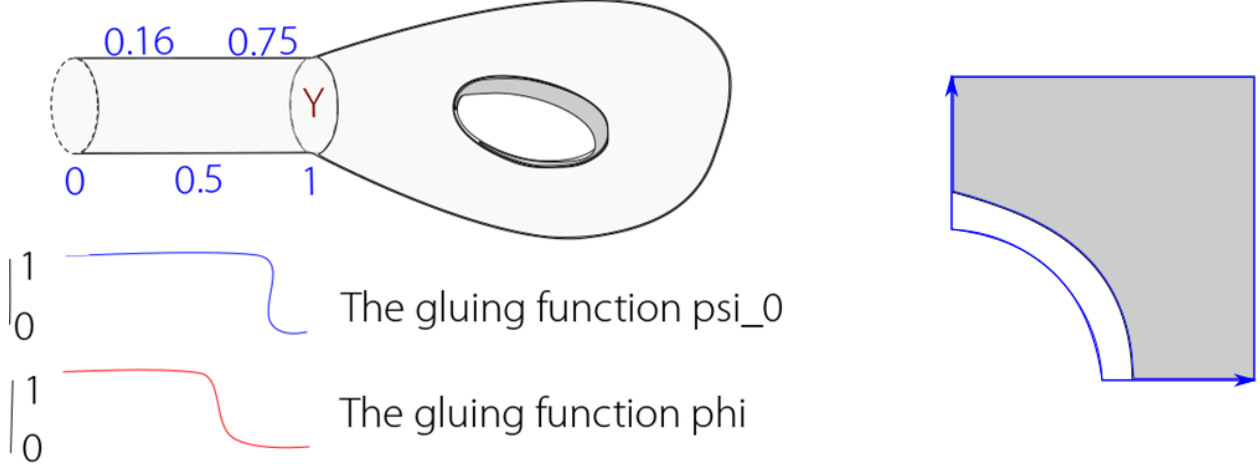
Figure 12: Left: compatible cutoffs separate the compact interior from the product cylinder while retaining an overlap on which the two model kernels can be compared. Right: after lifting to the b-double space, the boundary correction is supported near the front face and away from the opposite side face. This support control makes the alternating temporal and boundary corrections compatible.
